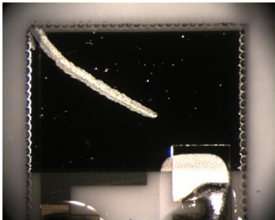
Sensor with a scratch
